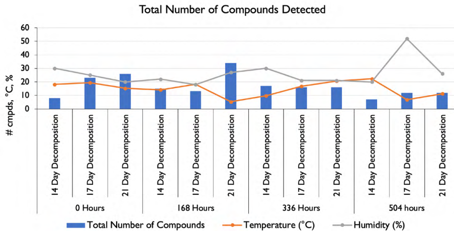
Figure 12. Total number of compounds detected in relation to average temperature and humidity.
