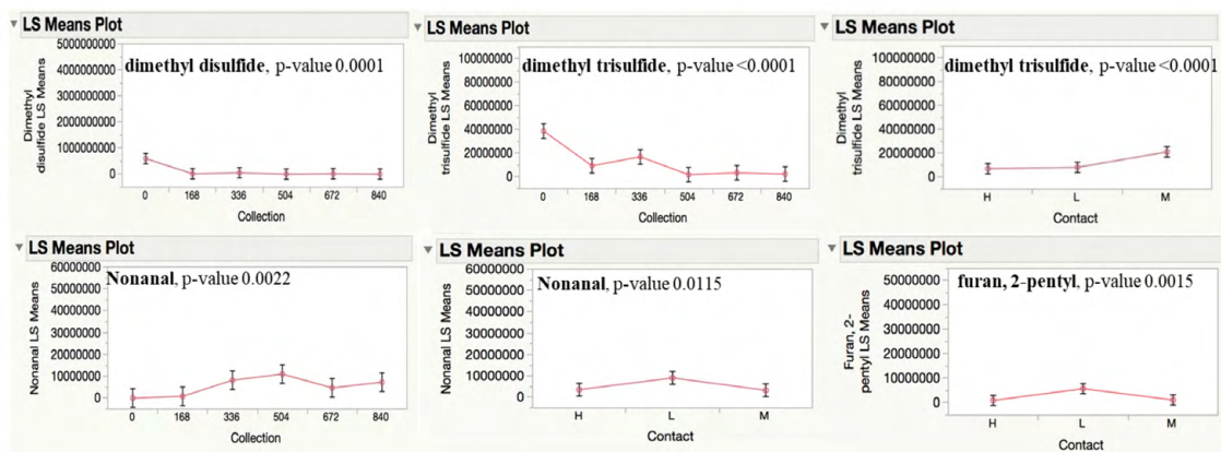
Figure 9. A Multi-factorial ANOVA Results for High Frequency Compounds – Meat Simulation Mode.
